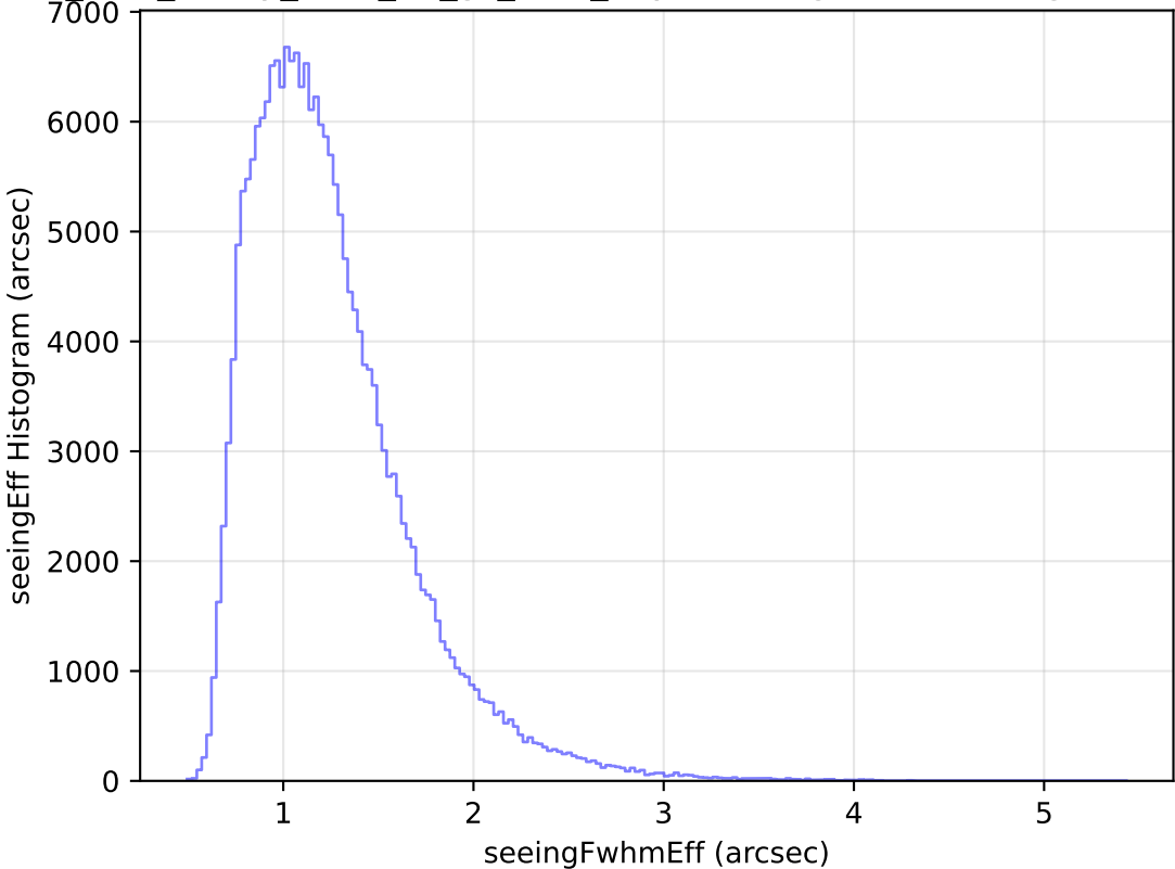
too_elab_heavy_r128_d3_gz_v3.4_10yrs WFD g band: seeingEff Histogram
