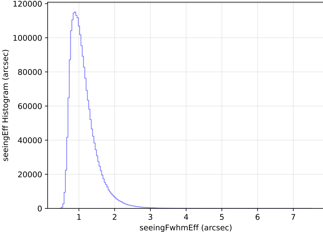
too_elab_heavy_r128_d3_gz_v3.4_10yrs WFD all bands: seeingEff Histogram
