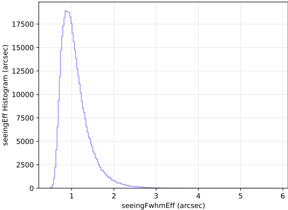
too_elab_heavy_r128_d3_gz_v3.4_10yrs All sky z band: seeingEff Histogram
