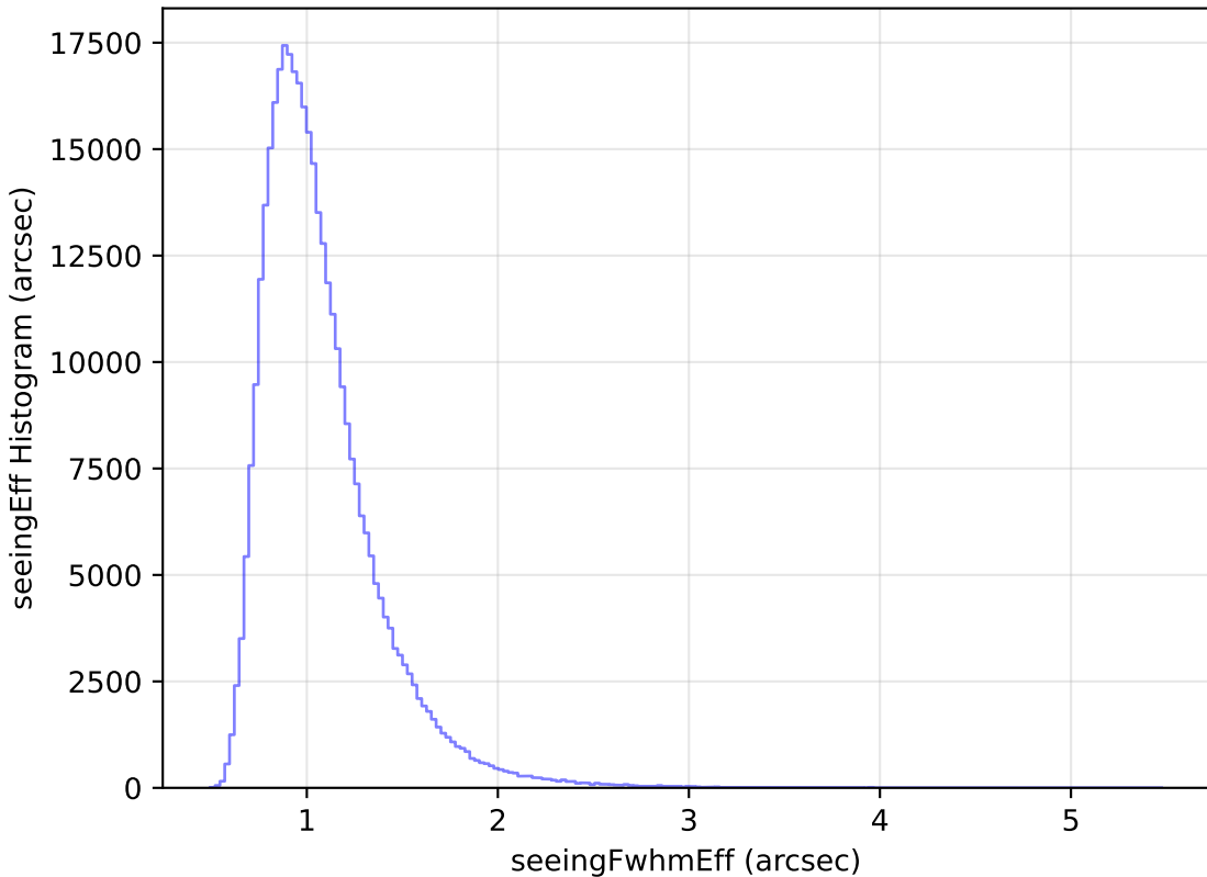
too_elab_heavy_r128_d3_gz_v3.4_10yrs All sky y band: seeingEff Histogram
