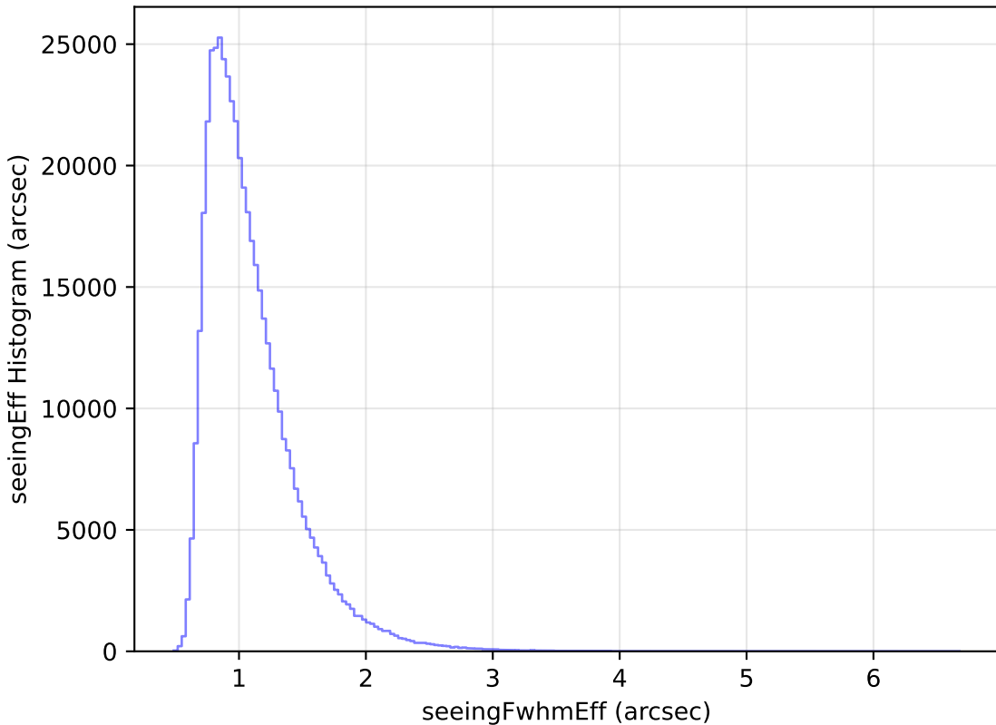
too_elab_heavy_r128_d3_gz_v3.4_10yrs All sky i band: seeingEff Histogram
