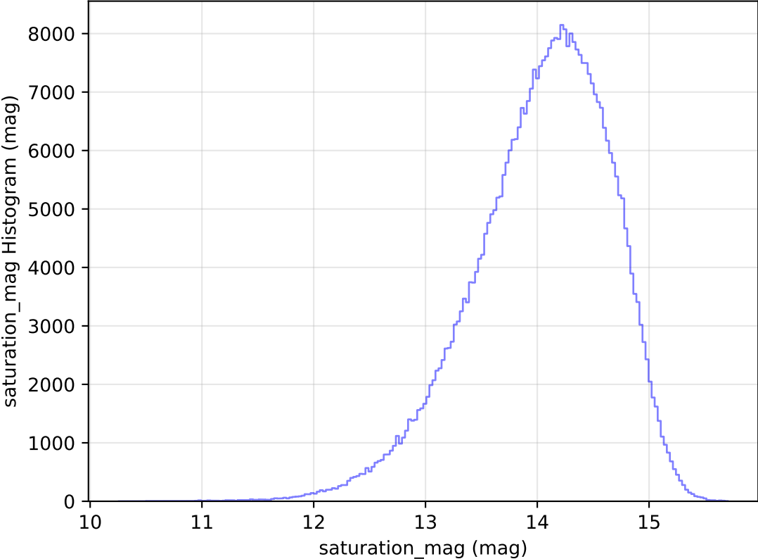
too_elab_heavy_r128_d3_gz_v3.4_10yrs WFD z band: saturation_mag Histogram
