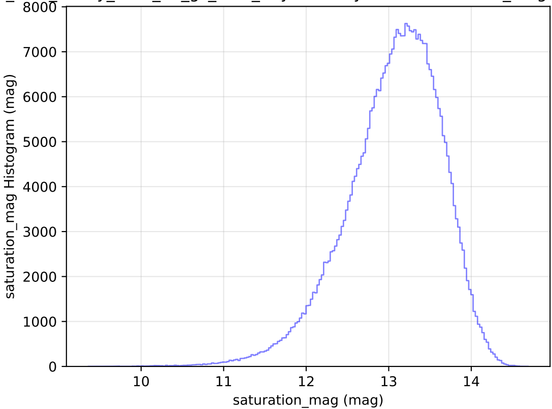
too_elab_heavy_r128_d3_gz_v3.4_10yrs WFD y band: saturation_mag Histogram
