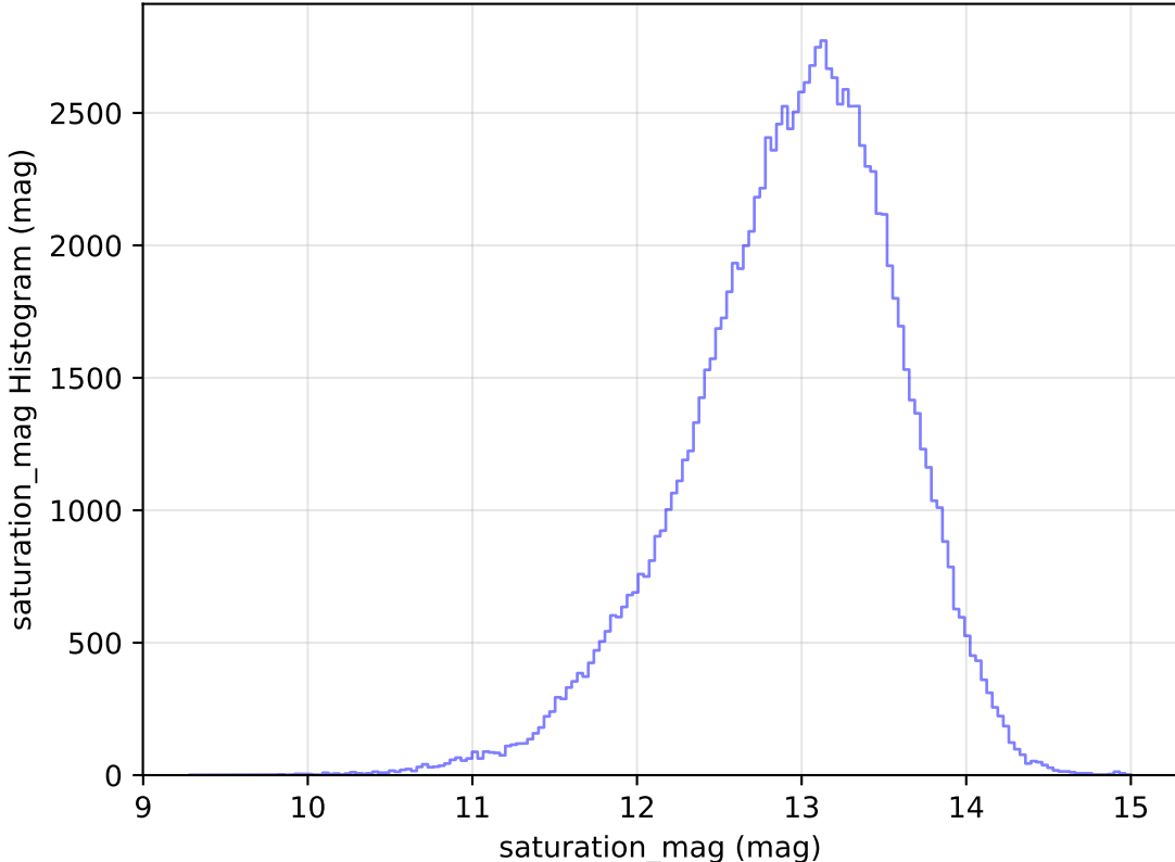
too_elab_heavy_r128_d3_gz_v3.4_10yrs WFD u band: saturation_mag Histogram
