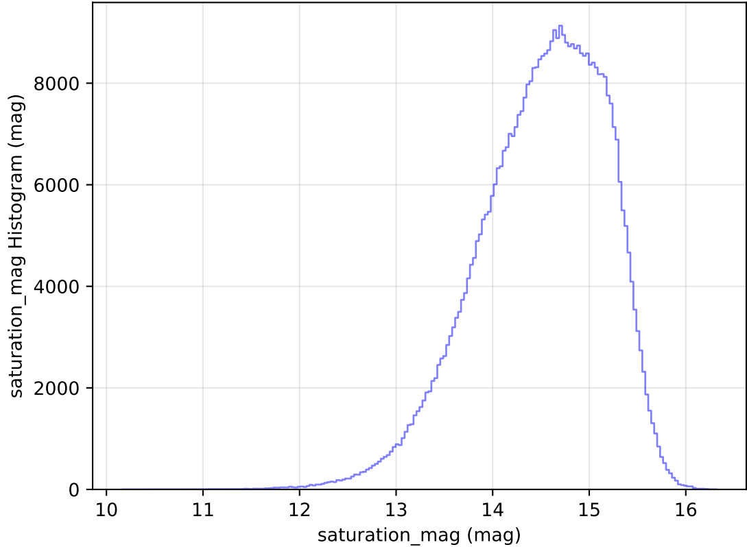
too_elab_heavy_r128_d3_gz_v3.4_10yrs WFD r band: saturation_mag Histogram
