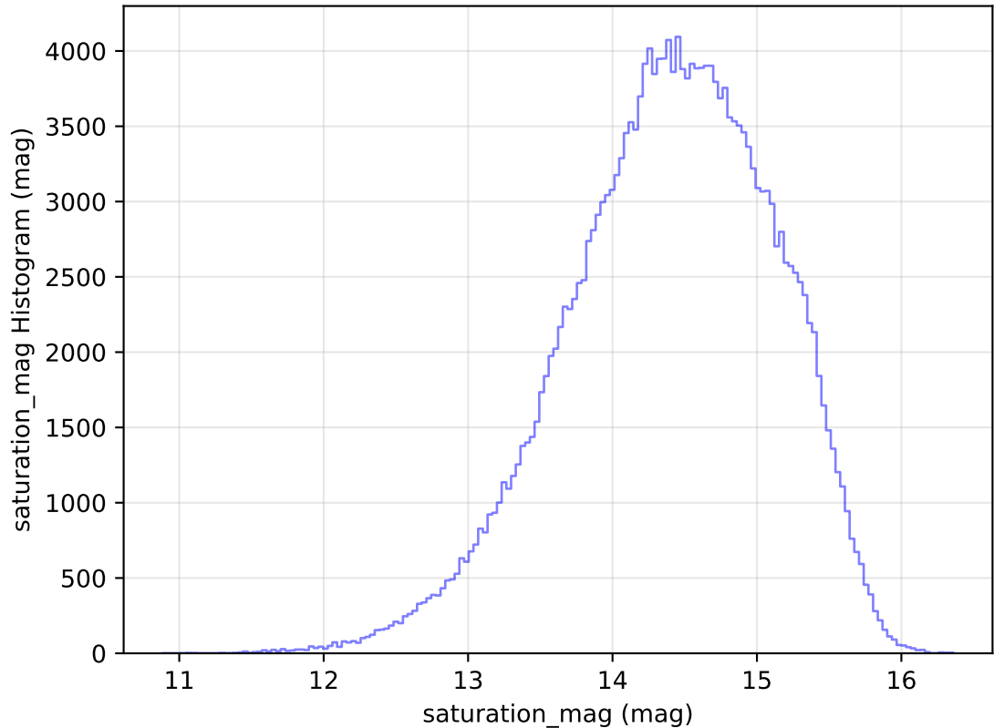
too_elab_heavy_r128_d3_gz_v3.4_10yrs WFD g band: saturation_mag Histogram
