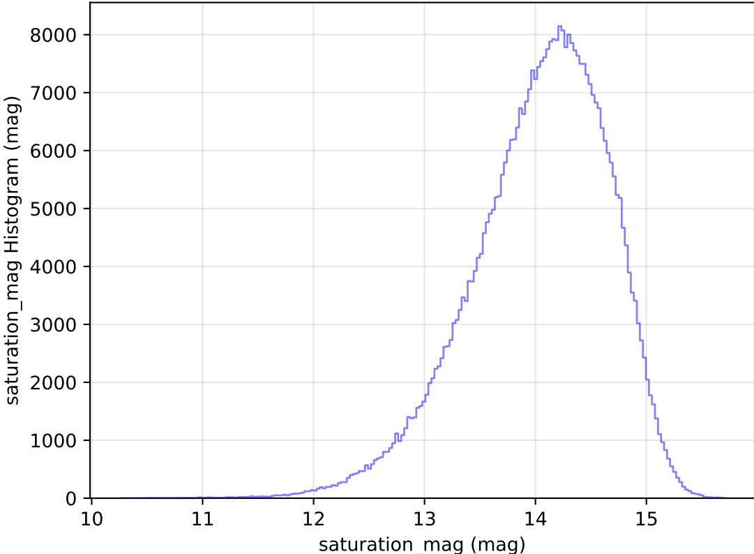
too_elab_heavy_r128_d3_gz_v3.4_10yrs All sky z band: saturation_mag Histogram
