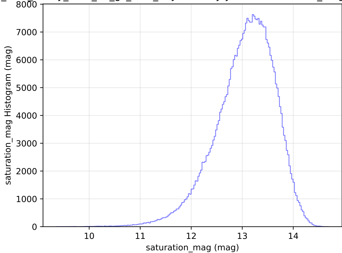
too_elab_heavy_r128_d3_gz_v3.4_10yrs All sky y band: saturation_mag Histogram
