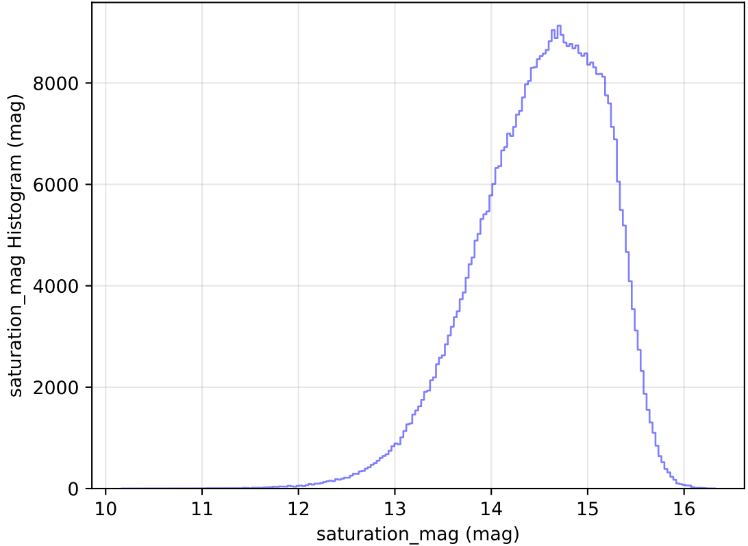
too_elab_heavy_r128_d3_gz_v3.4_10yrs All sky r band: saturation_mag Histogram
