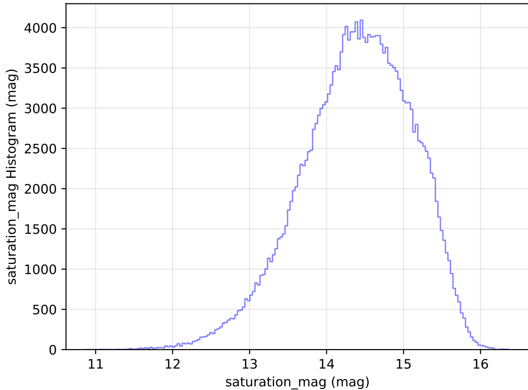
too_elab_heavy_r128_d3_gz_v3.4_10yrs All sky g band: saturation_mag Histogram
