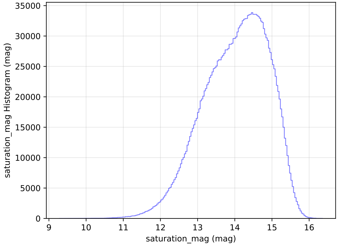
too_elab_heavy_r128_d3_gz_v3.4_10yrs All sky all bands: saturation_mag Histogram
