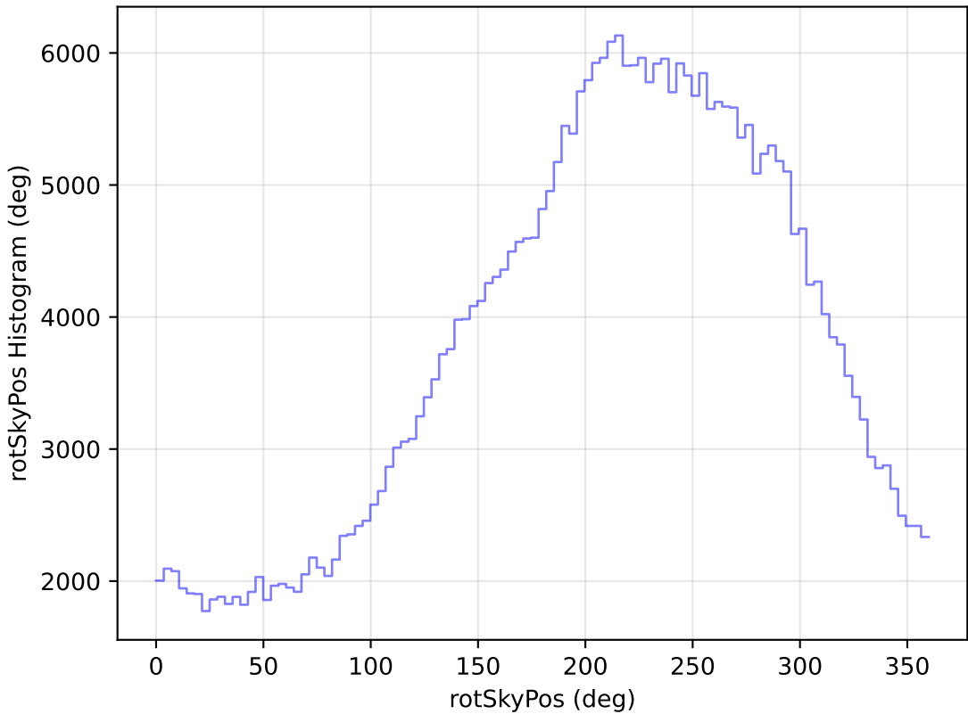
too_elab_heavy_r128_d3_gz_v3.4_10yrs WFD y band: rotSkyPos Histogram
