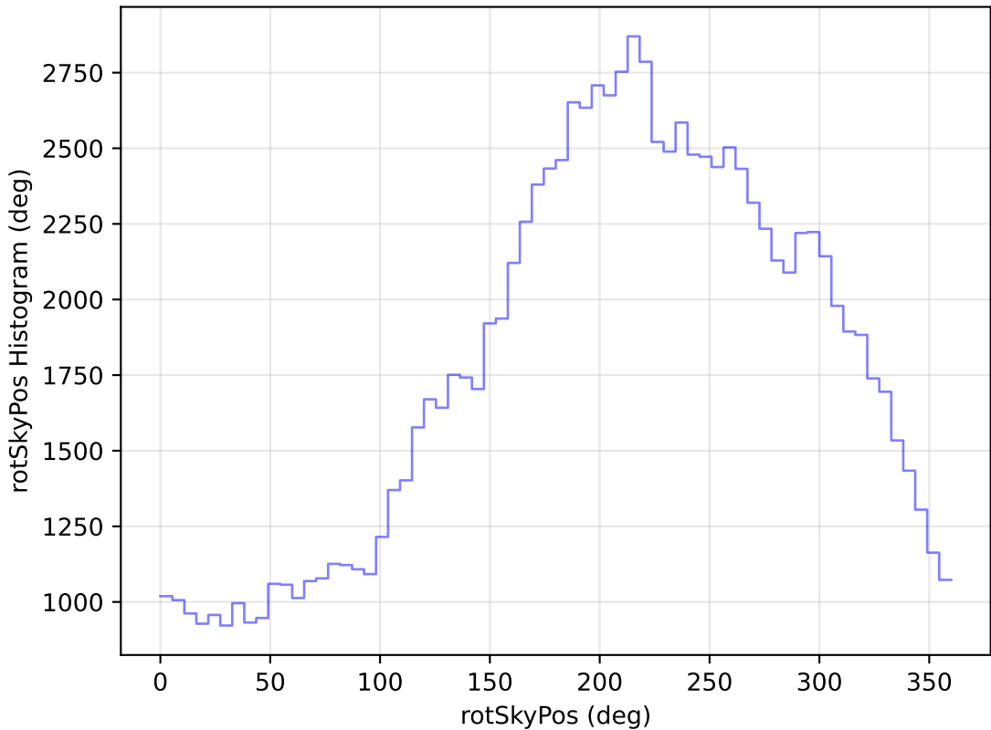
too_elab_heavy_r128_d3_gz_v3.4_10yrs WFD u band: rotSkyPos Histogram
