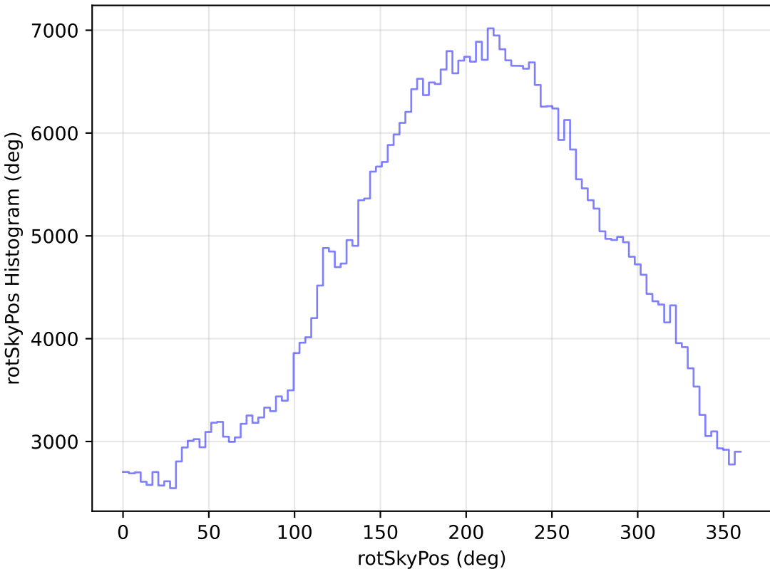
too_elab_heavy_r128_d3_gz_v3.4_10yrs WFD r band: rotSkyPos Histogram
