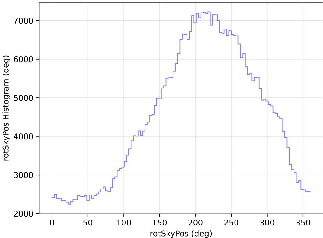
too_elab_heavy_r128_d3_gz_v3.4_10yrs WFD i band: rotSkyPos Histogram
