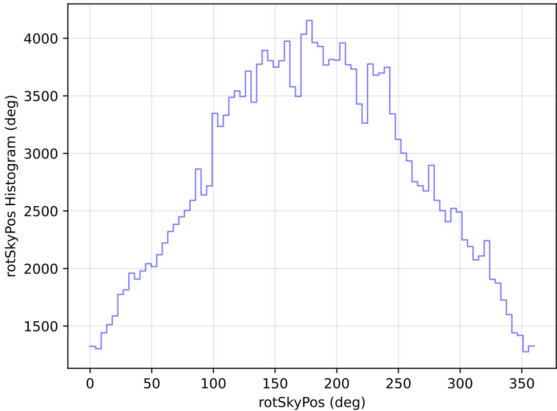
too_elab_heavy_r128_d3_gz_v3.4_10yrs WFD g band: rotSkyPos Histogram
