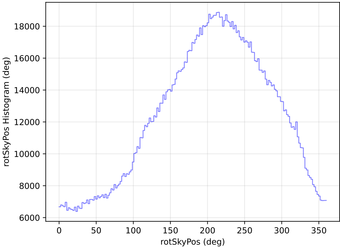
too_elab_heavy_r128_d3_gz_v3.4_10yrs WFD all bands: rotSkyPos Histogram
