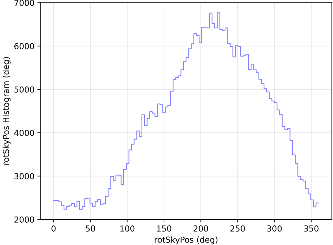
too_elab_heavy_r128_d3_gz_v3.4_10yrs All sky z band: rotSkyPos Histogram
