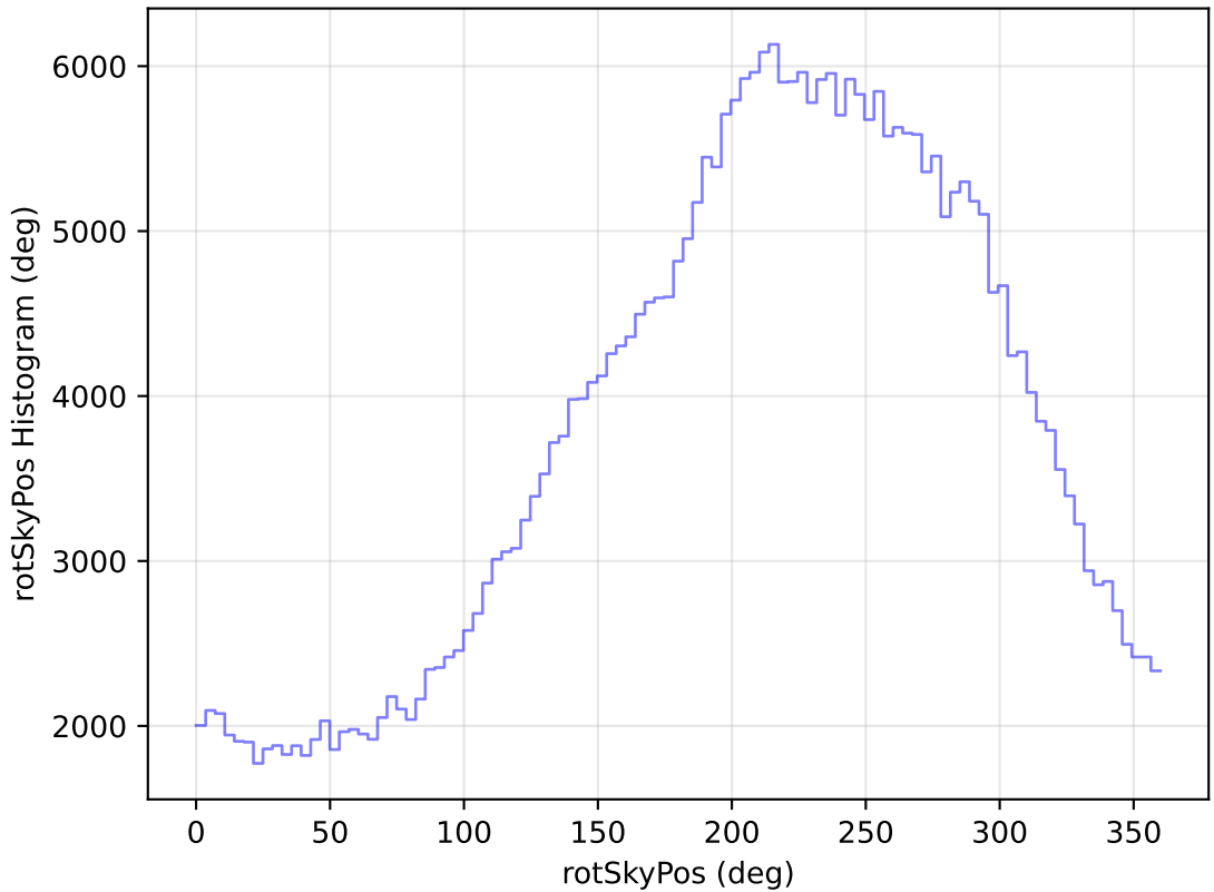
too_elab_heavy_r128_d3_gz_v3.4_10yrs All sky y band: rotSkyPos Histogram
