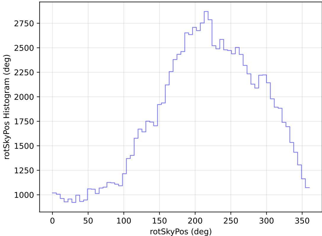
too_elab_heavy_r128_d3_gz_v3.4_10yrs All sky u band: rotSkyPos Histogram
