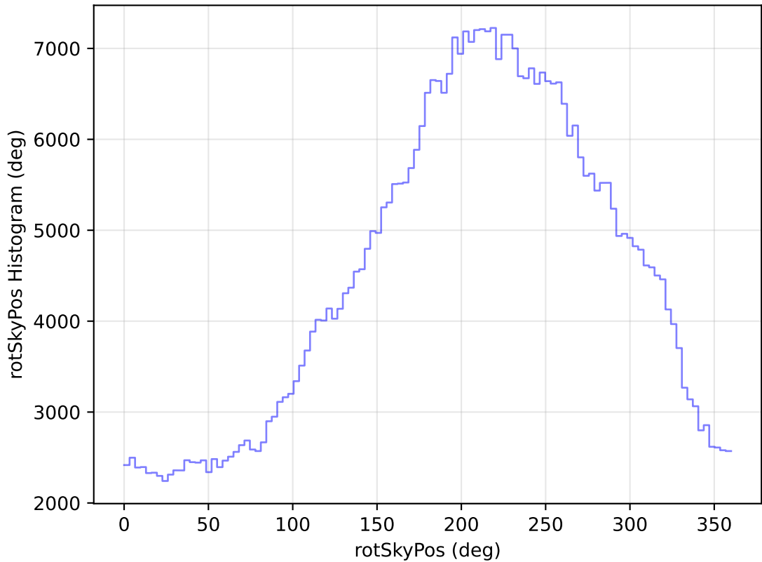
too_elab_heavy_r128_d3_gz_v3.4_10yrs All sky i band: rotSkyPos Histogram
