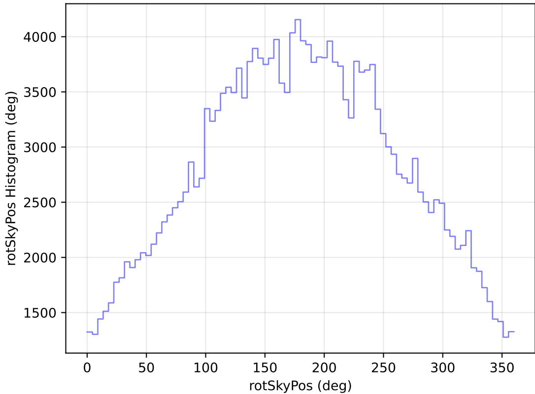
too_elab_heavy_r128_d3_gz_v3.4_10yrs All sky g band: rotSkyPos Histogram
