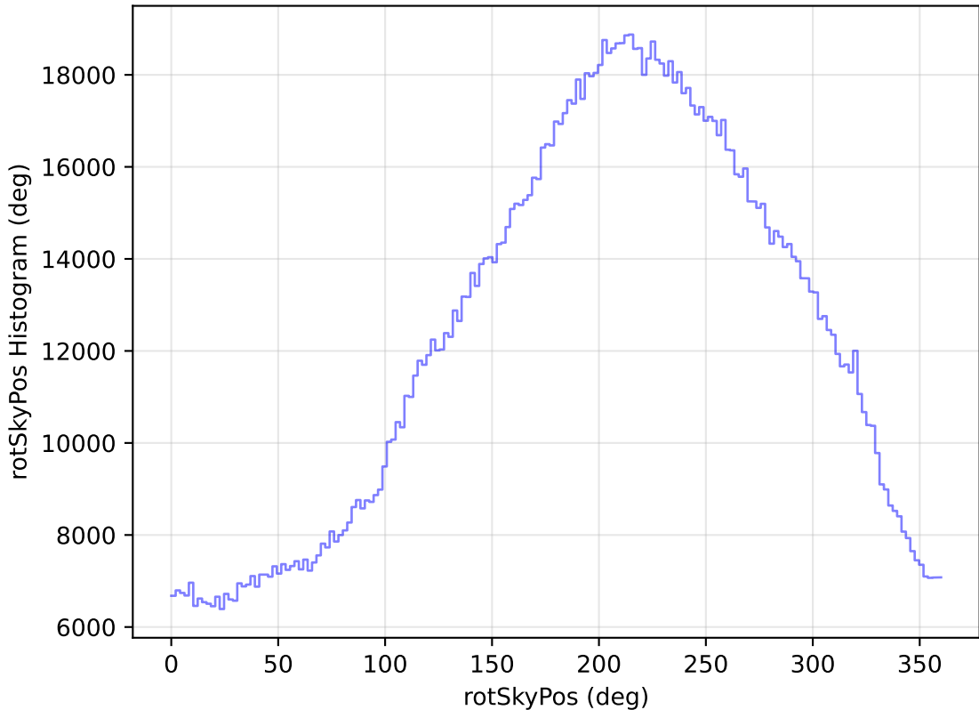
too_elab_heavy_r128_d3_gz_v3.4_10yrs All sky all bands: rotSkyPos Histogram
