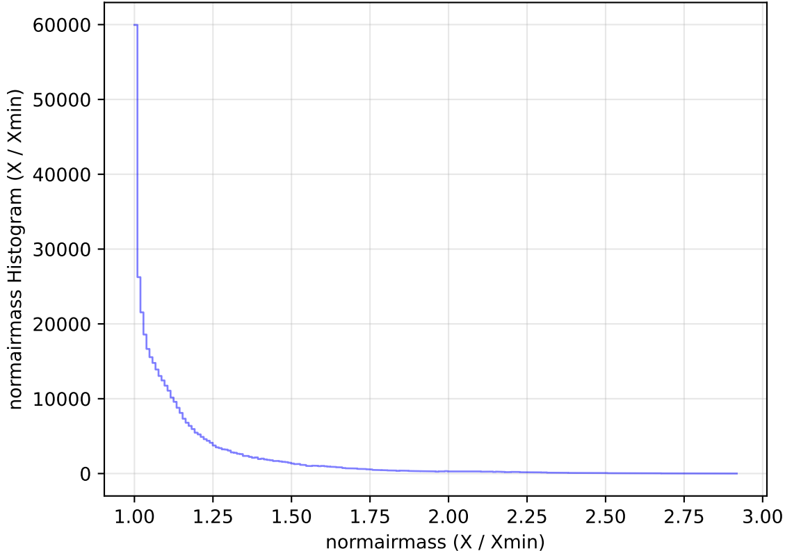
too_elab_heavy_r128_d3_gz_v3.4_10yrs WFD z band: normairmass Histogram
