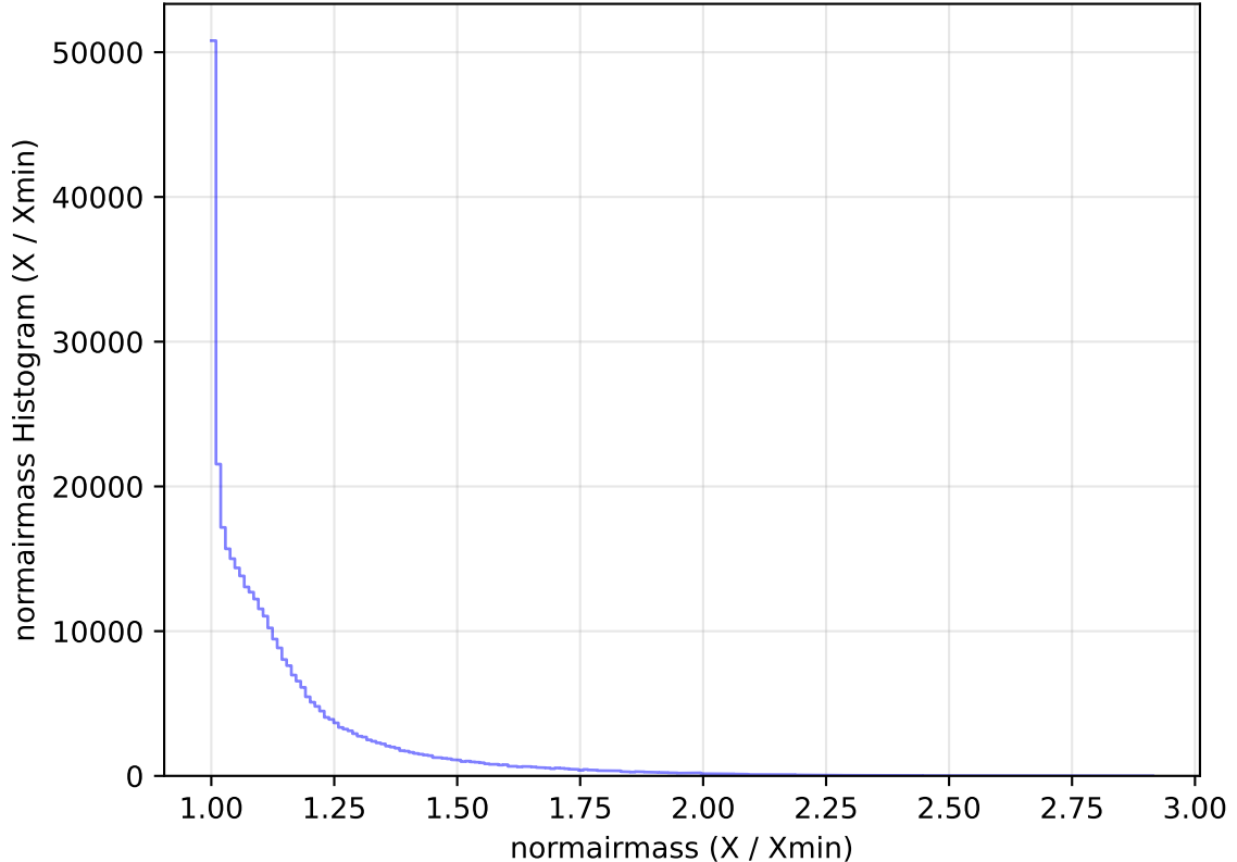
too_elab_heavy_r128_d3_gz_v3.4_10yrs WFD y band: normairmass Histogram
