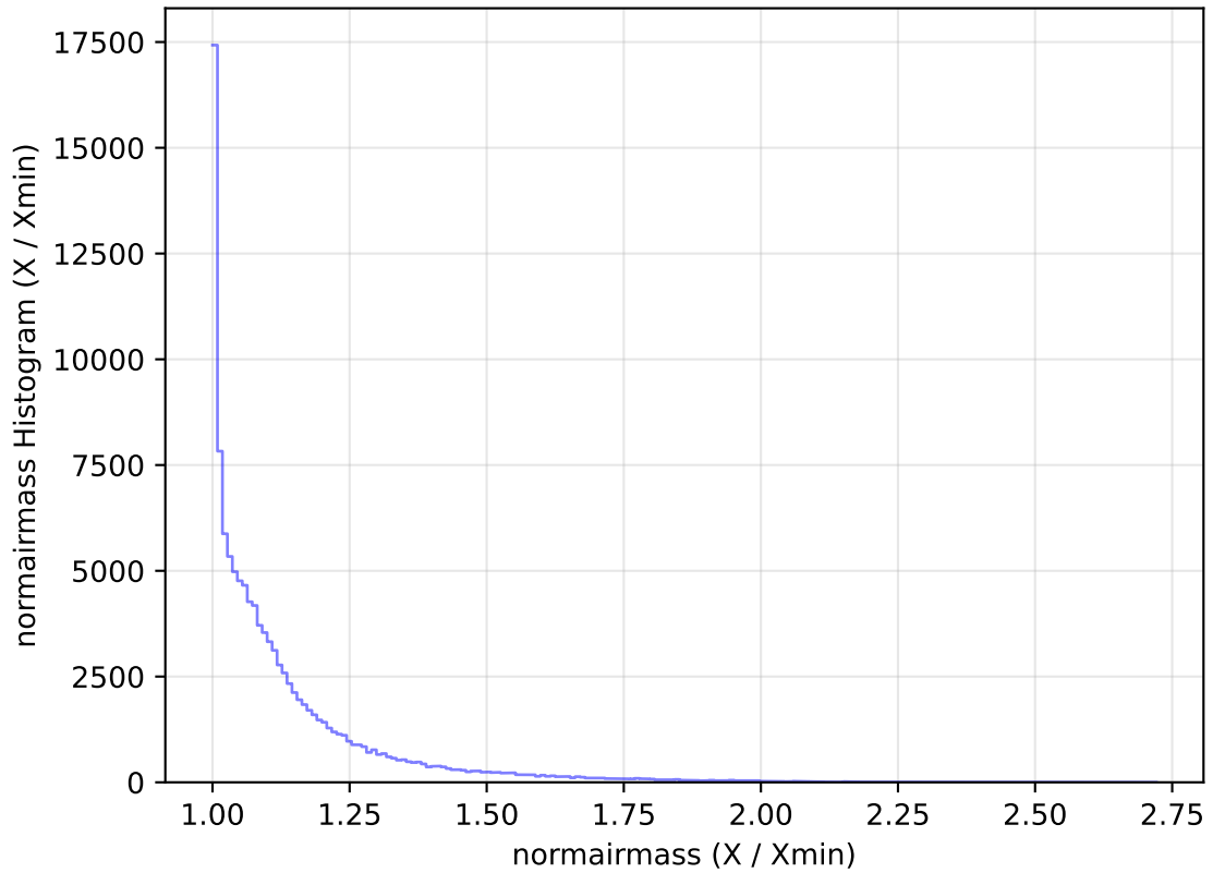
too_elab_heavy_r128_d3_gz_v3.4_10yrs WFD u band: normairmass Histogram
