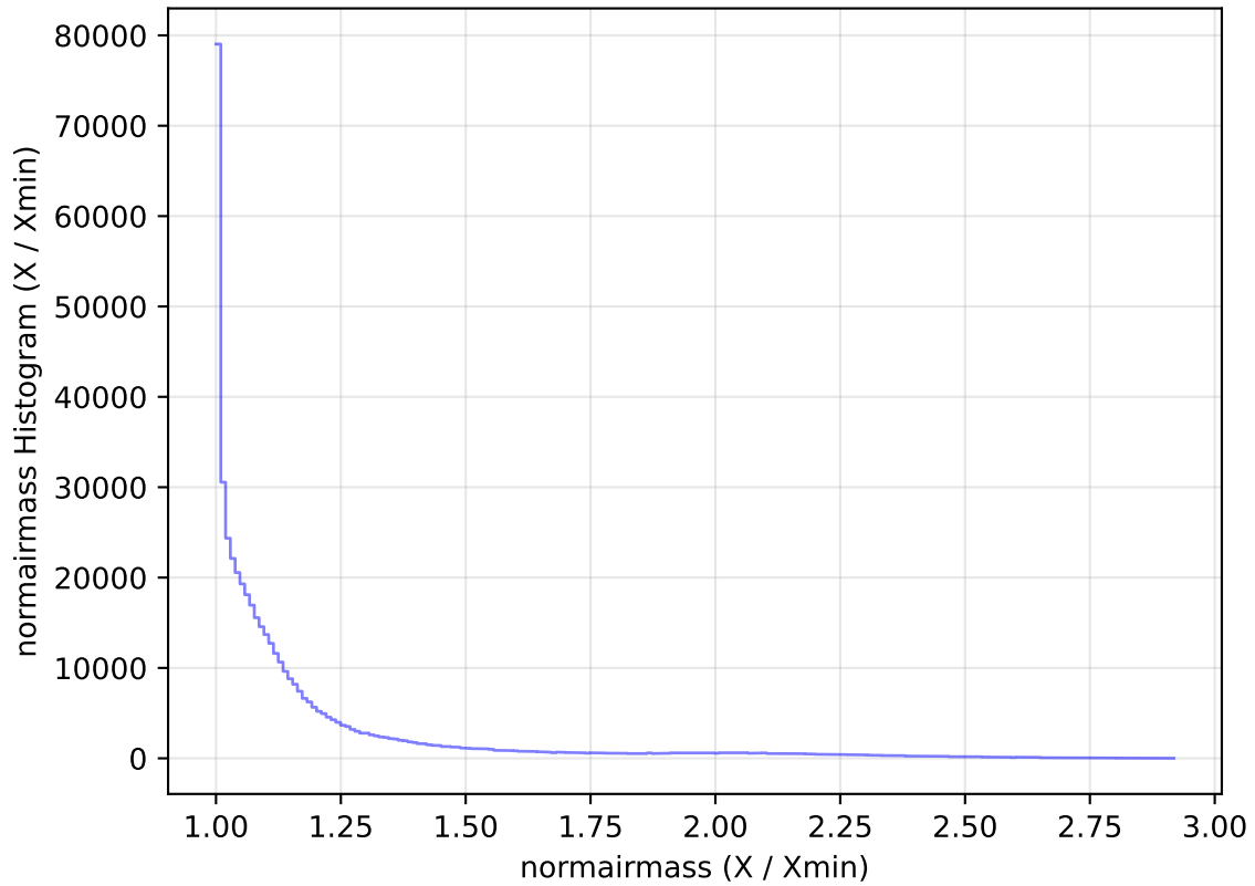
too_elab_heavy_r128_d3_gz_v3.4_10yrs WFD i band: normairmass Histogram
