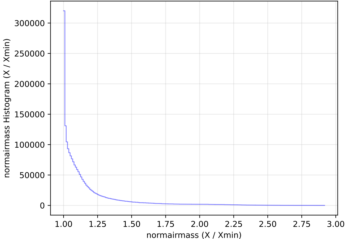
too_elab_heavy_r128_d3_gz_v3.4_10yrs WFD all bands: normairmass Histogram
