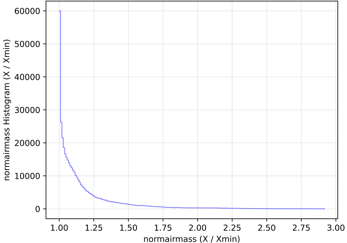
too_elab_heavy_r128_d3_gz_v3.4_10yrs All sky z band: normairmass Histogram
