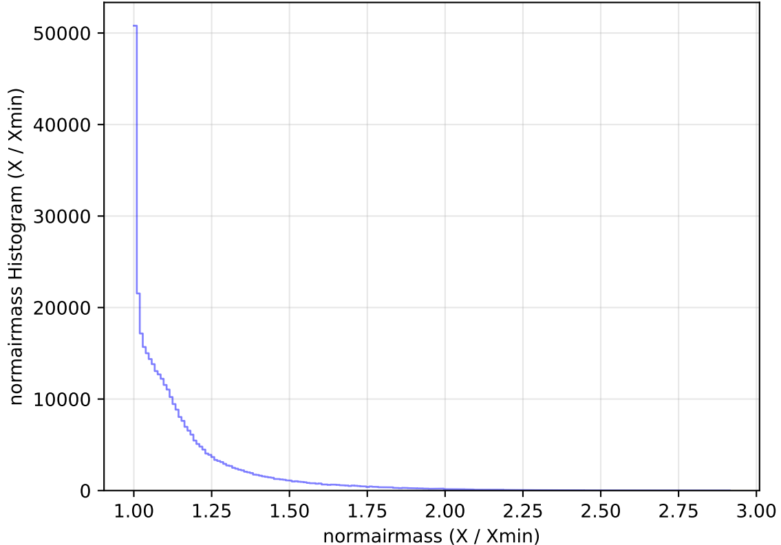
too_elab_heavy_r128_d3_gz_v3.4_10yrs All sky y band: normairmass Histogram
