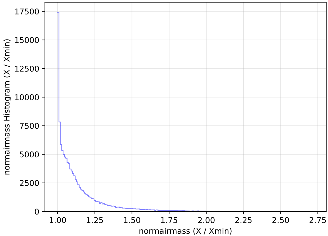
too_elab_heavy_r128_d3_gz_v3.4_10yrs All sky u band: normairmass Histogram
