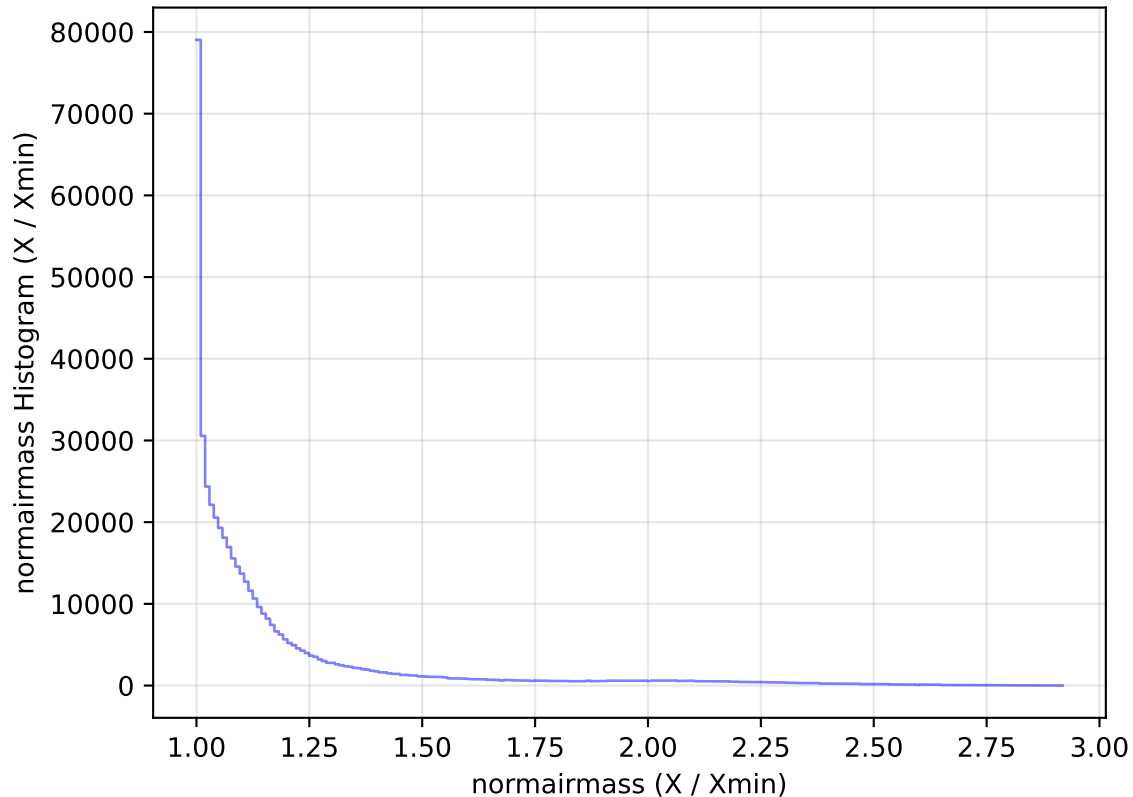
too_elab_heavy_r128_d3_gz_v3.4_10yrs All sky i band: normairmass Histogram
