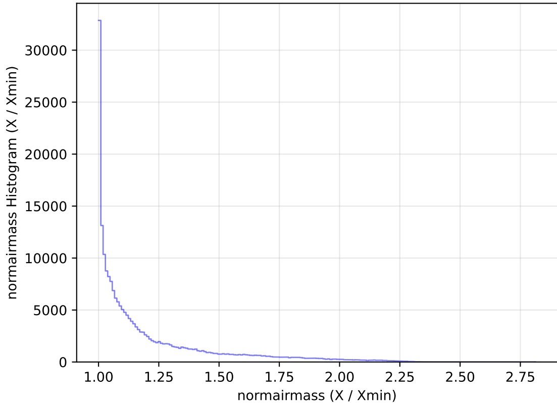
too_elab_heavy_r128_d3_gz_v3.4_10yrs All sky g band: normairmass Histogram
