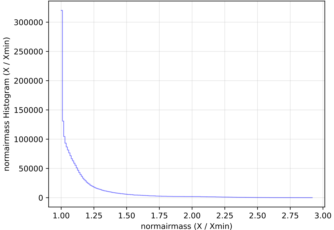
too_elab_heavy_r128_d3_gz_v3.4_10yrs All sky all bands: normairmass Histogram
