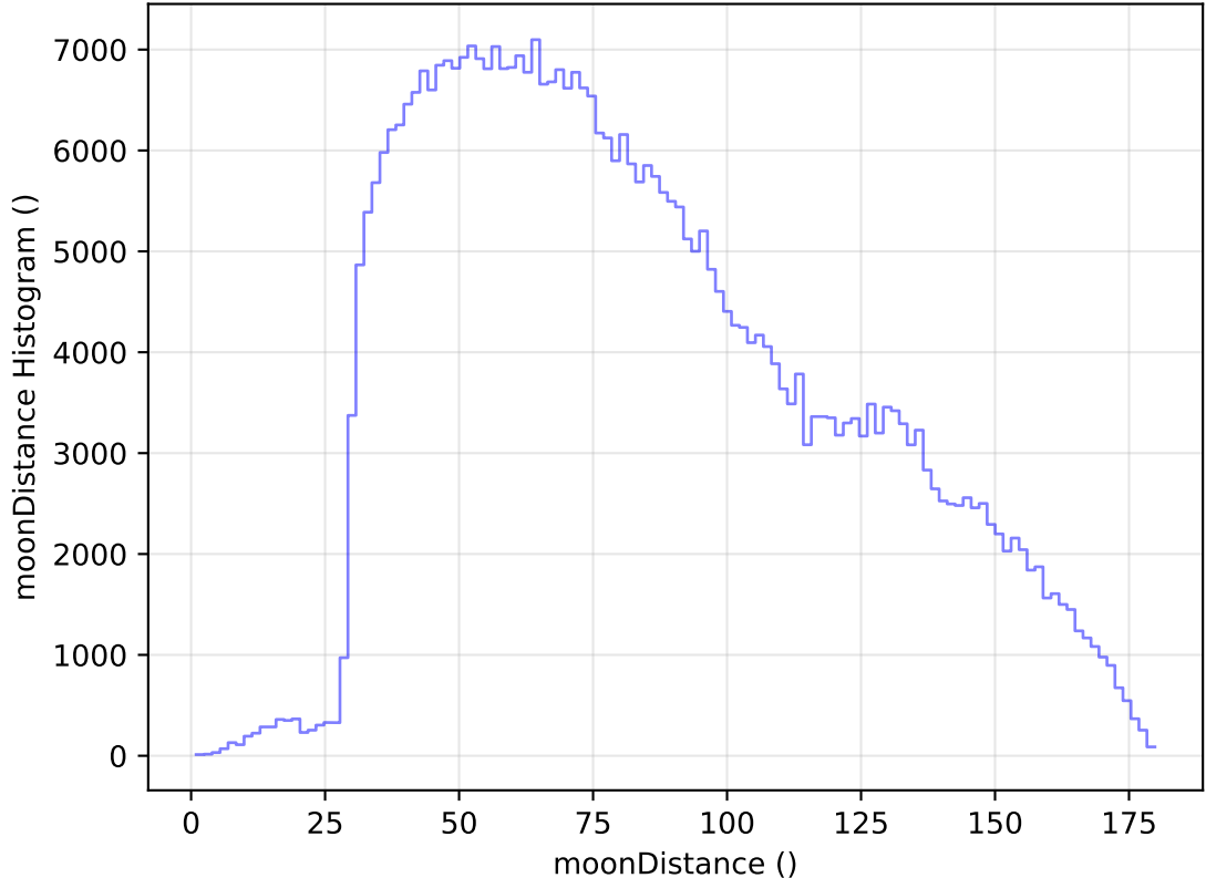
too_elab_heavy_r128_d3_gz_v3.4_10yrs WFD z band: moonDistance Histogram
