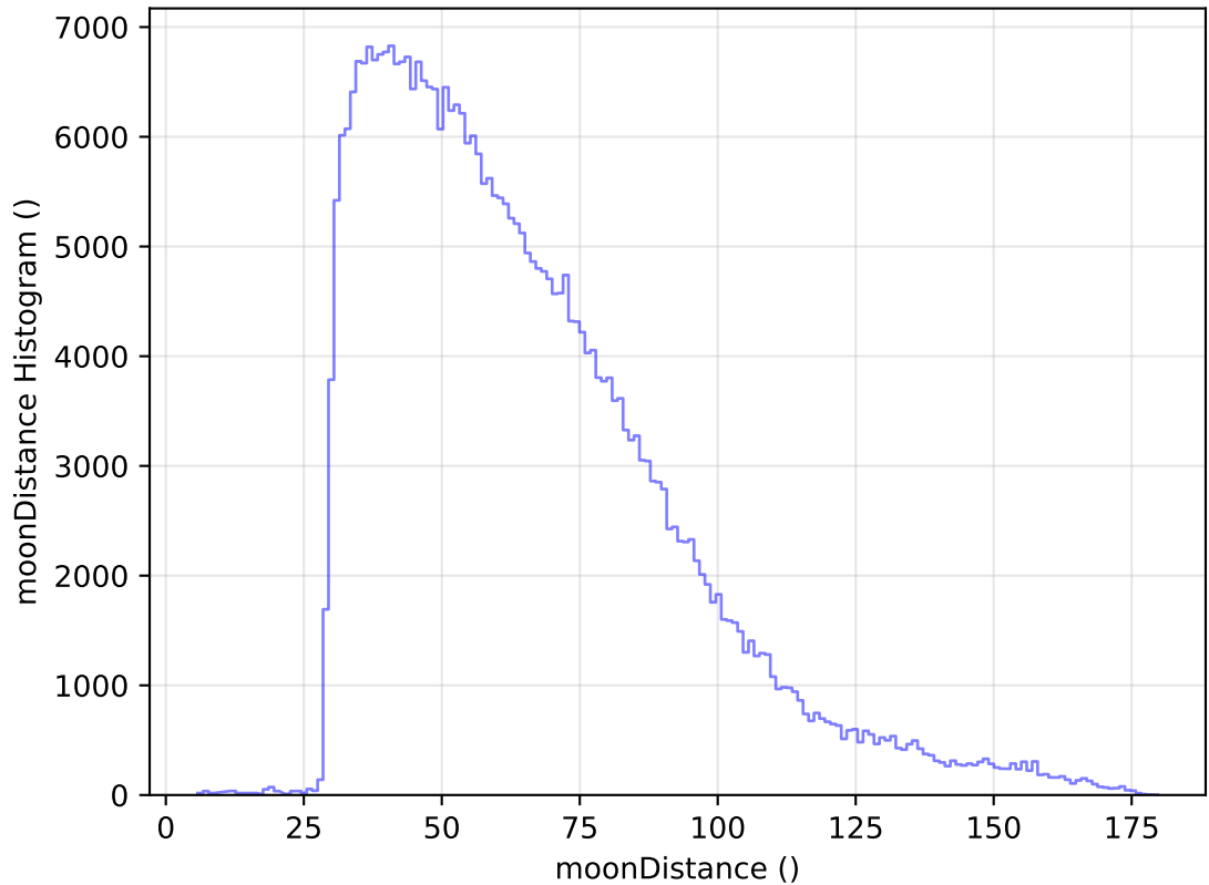
too_elab_heavy_r128_d3_gz_v3.4_10yrs WFD y band: moonDistance Histogram
