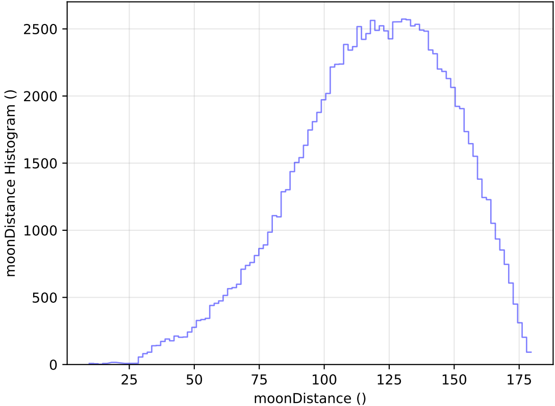
too_elab_heavy_r128_d3_gz_v3.4_10yrs WFD u band: moonDistance Histogram
