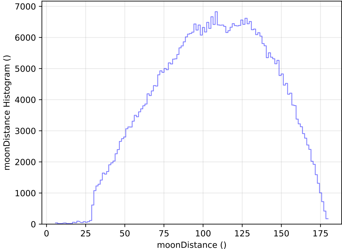
too_elab_heavy_r128_d3_gz_v3.4_10yrs WFD r band: moonDistance Histogram
