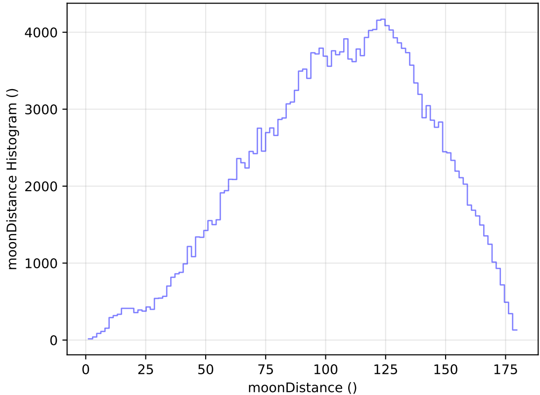
too_elab_heavy_r128_d3_gz_v3.4_10yrs WFD g band: moonDistance Histogram
