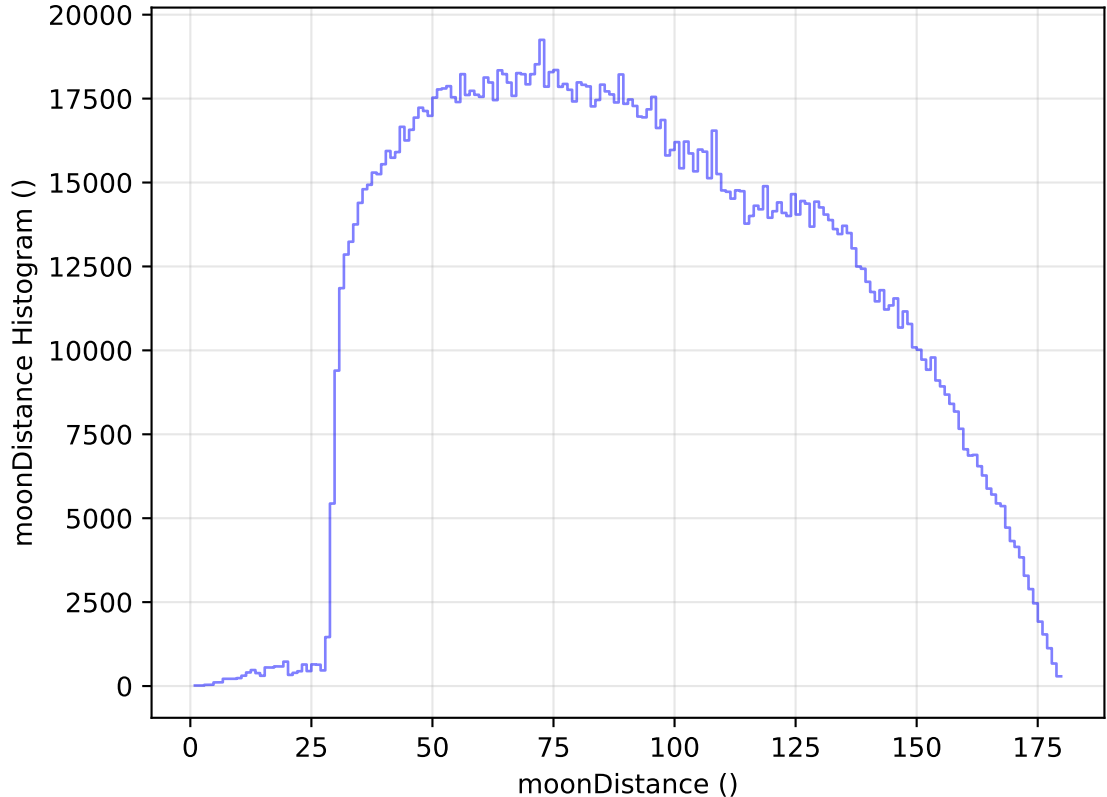
too_elab_heavy_r128_d3_gz_v3.4_10yrs WFD all bands: moonDistance Histogram
