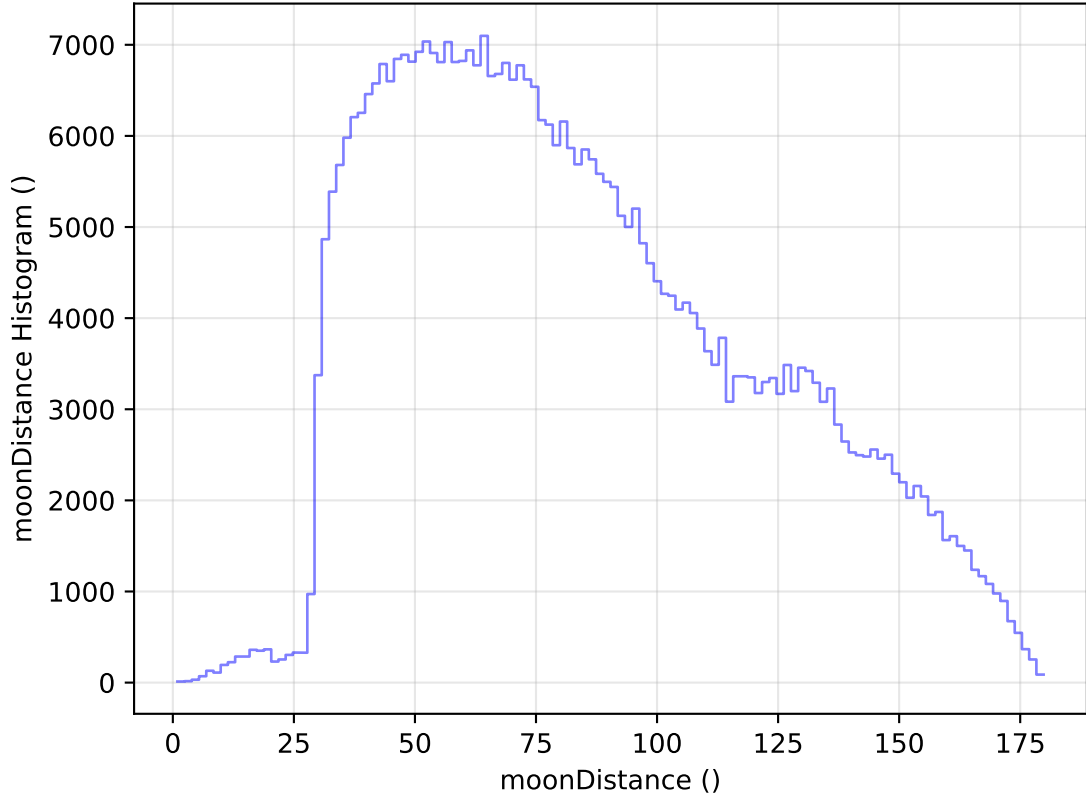
too_elab_heavy_r128_d3_gz_v3.4_10yrs All sky z band: moonDistance Histogram
