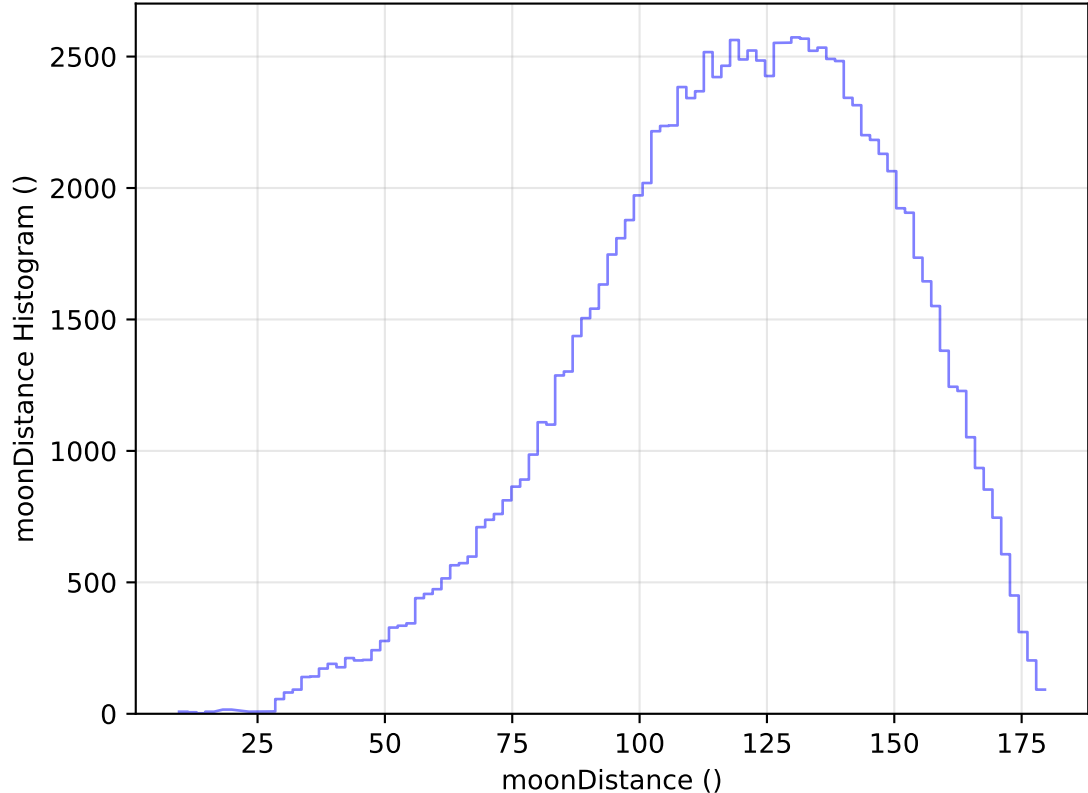
too_elab_heavy_r128_d3_gz_v3.4_10yrs All sky u band: moonDistance Histogram
