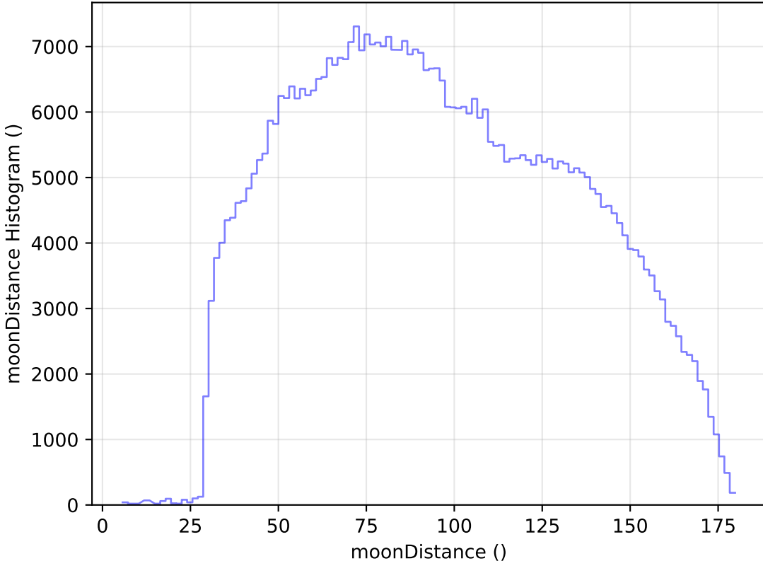
too_elab_heavy_r128_d3_gz_v3.4_10yrs All sky i band: moonDistance Histogram
