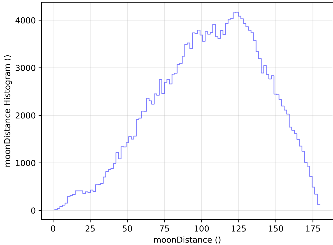
too_elab_heavy_r128_d3_gz_v3.4_10yrs All sky g band: moonDistance Histogram
