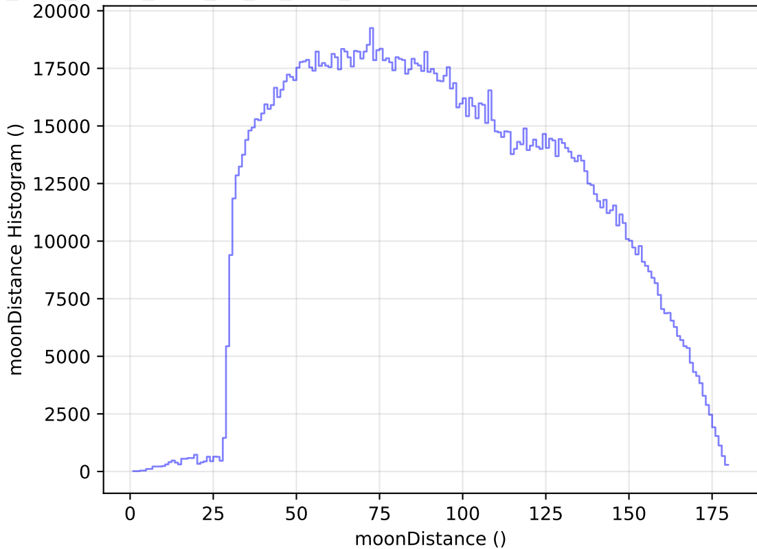
too_elab_heavy_r128_d3_gz_v3.4_10yrs All sky all bands: moonDistance Histogram
