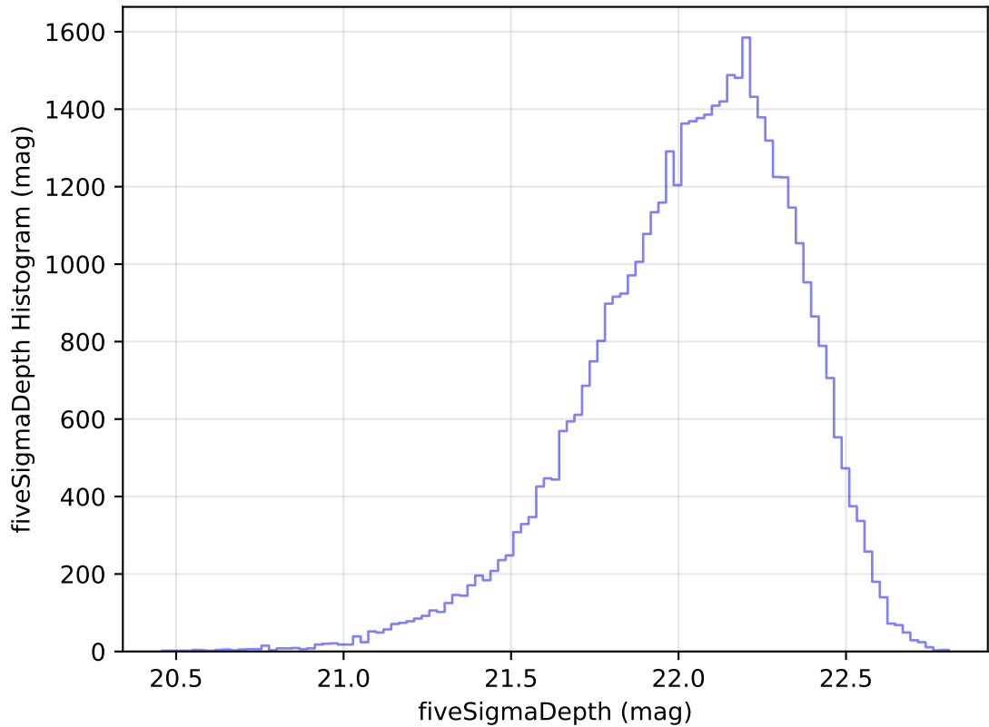
too_elab_heavy_r128_d3_gz_v3.4_10yrs Yr 1 y band: fiveSigmaDepth Histogram
